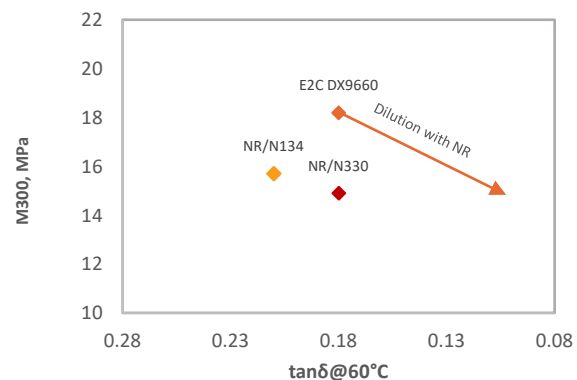
Figure 2. E2C DX9660 elastomer composite has high M300 and low hysteresis loss
